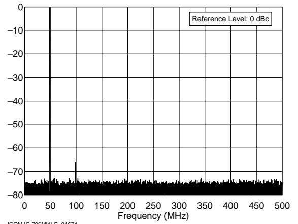
ICOM IC-706MkII G 01674 50.0 MHz Band, Spectral Purity, 100 W F:\SHARED\PROD_REV\TESTS\IC706G\IC706S6M.TXT
