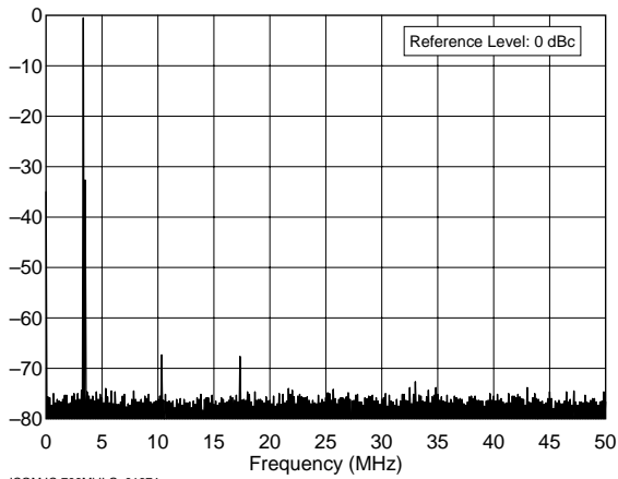
ICOM IC-706MkII G 01674 3.5 MHz Band, Spectral Purity, 100 W F:\SHARED\PROD_REV\TESTS\IC706G\IC706S80.TXT
