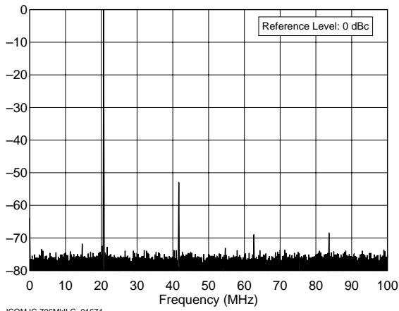
ICOM IC-706MkII G 01674 21.0 MHz Band, Spectral Purity, 100 W F:\SHARED\PROD_REV\TESTS\IC706G\IC706S15.TXT
