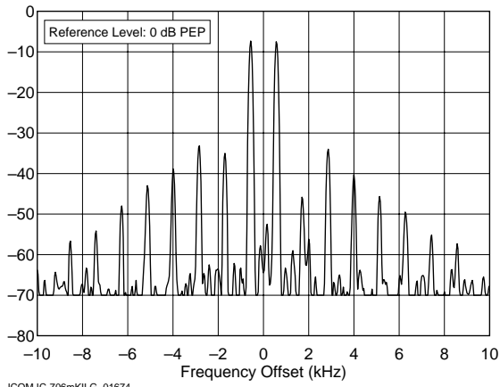
ICOM IC-706mKII G 01674 7.250 MHz, Transmit IMD, 100 W F:\SHARED\PROD_REVTESTS\IC706G\IC706I40.TXT
