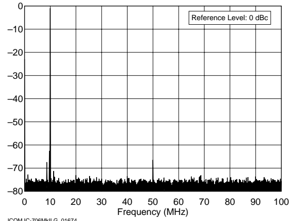
ICOM IC-706MkII G 01674 10.1 MHz Band, Spectral Purity, 100 W F:\SHARED\PROD_REV\TESTS\IC706G\IC706S30.TXT
