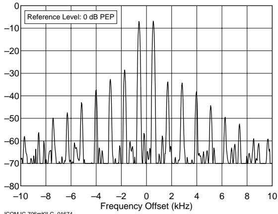
ICOM IC-706mKII G 01674 21.250 MHz, Transmit IMD, 100 W F:\SHARED\PROD_REV\TESTS\IC706G\IC706I15.TXT
