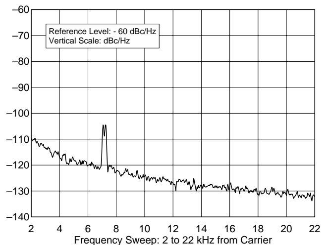
ICOM IC-706MkII G 01674 50.020 MHz, Phase Noise, 100 W F:\SHARED\PROD_REV\TESTS\IC706G\IC706P6M.TXT
