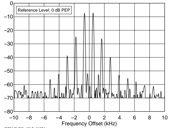
ICOM IC-706mKII G 01674 144.200 MHz, Transmit IMD, 50 W F:\SHARED\PROD_REV\TESTS\IC706G\IC706I2M.TXT
