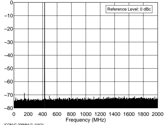
ICOM IC-706MkII G 01674 420.0 MHz Band, Spectral Purity, 20 W F:\SHARED\PROD_REV\TESTS\IC706G\IC706S70.TXT
