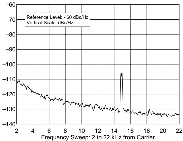
ICOM IC-706MkII G 01674 14.020 MHz, Phase Noise, 100 W F:\SHARED\PROD_REV\TESTS\IC706G\IC706P20.TXT
