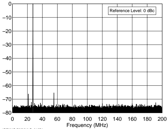
ICOM IC-706MkII G 01674 28.0 MHz Band, Spectral Purity, 100 W F:\SHARED\PROD_REV\TESTS\IC706G\IC706S10.TXT
