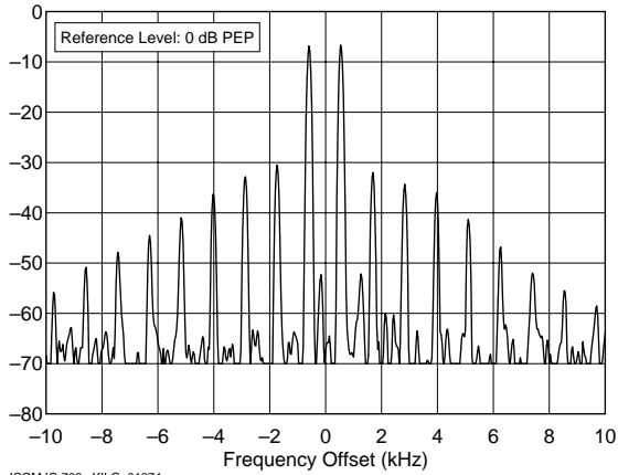
ICOM IC-706mKII G 01674 24.950 MHz, Transmit IMD, 100 W F:\SHARED\PROD_REV\TESTS\IC706G\IC706I12.TXT
