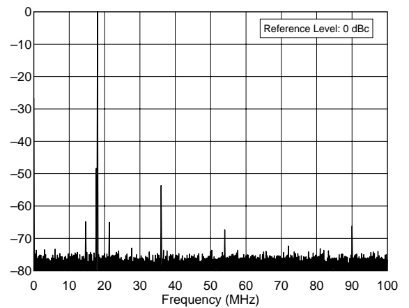
ICOM IC-706MkII G 01674 18.1 MHz Band, Spectral Purity, 100 W F:\SHARED\PROD_REV\TESTS\IC706G\IC706S17.TXT
