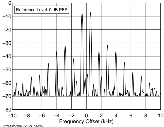
ICOM IC-706mKII G 01674 1.850 MHz, Transmit IMD, 100 W F:\SHARED\PROD_REVTESTS\IC706G\IC706I0.TXT
