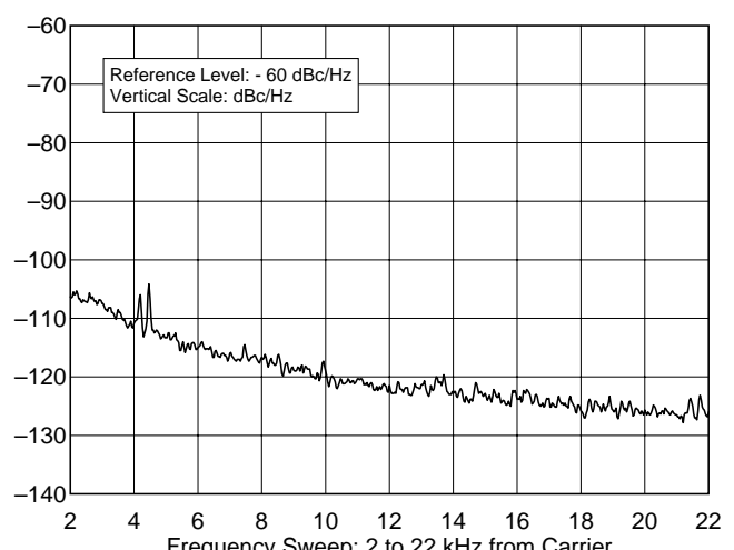
ICOM IC-706MkII G 01674 144.020 MHz, Phase Noise, 50 W F:\SHARED\PROD_REV\TESTS\IC706G\IC706P2M.TXT
