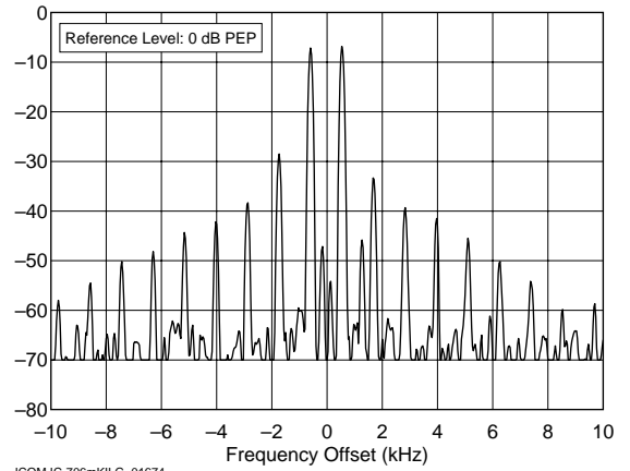
ICOM IC-706mKII G 01674 50.200 MHz, Transmit IMD, 100 W F:\SHARED\PROD_REV\TESTS\IC706G\IC706I6M.TXT
