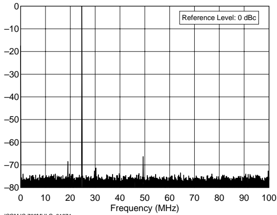
ICOM IC-706MkII G 01674 24.9 MHz Band, Spectral Purity, 100 W F:\SHARED\PROD_REV\TESTS\IC706G\IC706S12.TXT
