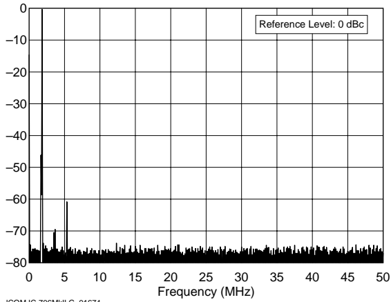
ICOM IC-706MkII G 01674 1.8 MHz Band, Spectral Purity, 100 W F:\SHARED\PROD_REV\TESTS\IC706G\IC706SLO.TXT
