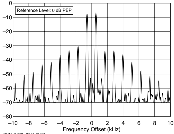
ICOM IC-706mKII G 01674 28.350 MHz, Transmit IMD, 100 W F:\SHARED\PROD_REV\TESTS\IC706G\IC706I10.TXT
