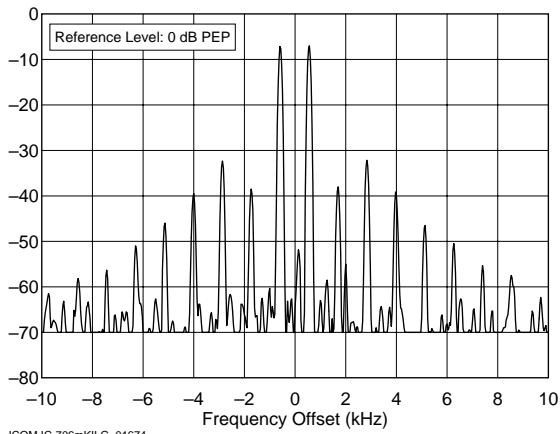
ICOM IC-706mKII G 01674 3.900 MHz, Transmit IMD, 100 W F:\SHARED\PROD_REVTESTS\IC706G\IC706I80.TXT
