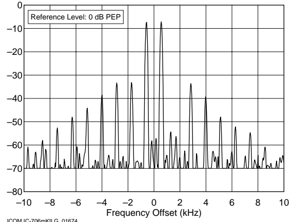
ICOM IC-706mKII G 01674 10.120 MHz, Transmit IMD, 100 W F:\SHARED\PROD_REVTESTS\IC706G\IC706I30.TXT
