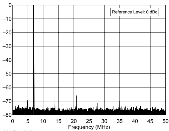
ICOM IC-706MkII G 01674 7.0 MHz Band, Spectral Purity, 100 W F:\SHARED\PROD_REV\TESTS\IC706G\IC706S40.TXT
