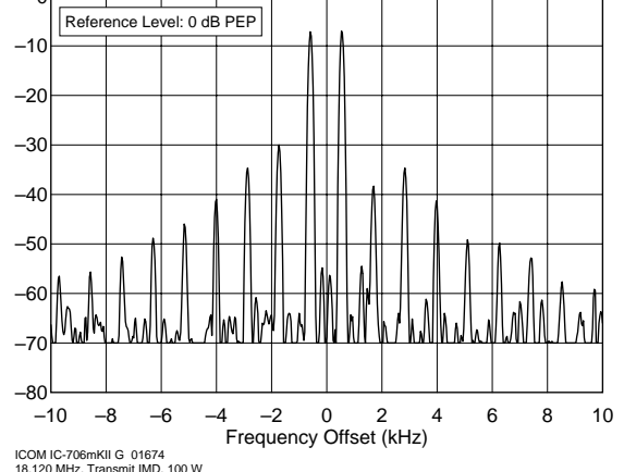
ICOM IC-706mKII G 01674 18.120 MHz, Transmit IMD, 100 W F:\SHARED\PROD_REVTESTS\IC706G\IC706I17.TXT
