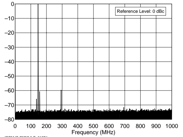
ICOM IC-706MkII G 01674 144.0 MHz Band, Spectral Purity, 50 W F:\SHARED\PROD_REV\TESTS\IC706G\IC706S2M.TXT
