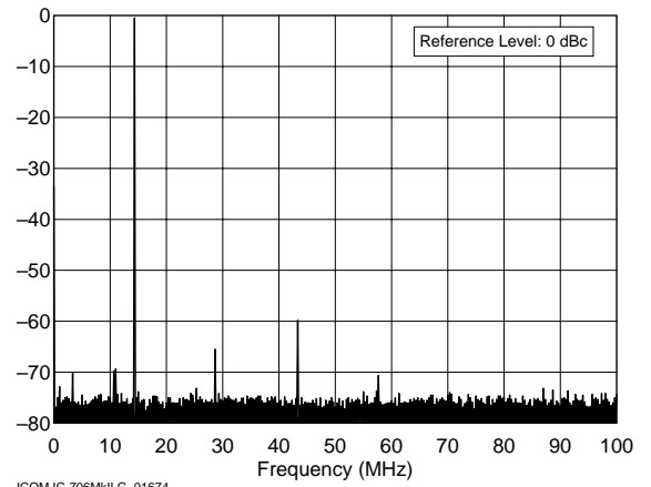
ICOM IC-706MkII G 01674 14.0 MHz Band, Spectral Purity, 100 W F:\SHARED\PROD_REV\TESTS\IC706G\IC706S20.TXT
