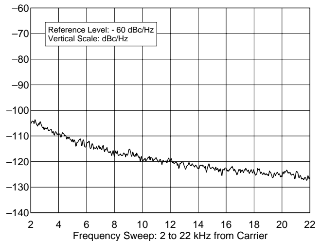
ICOM IC-706MkII G 01674 432.020 MHz, Phase Noise, 20 W F:\SHARED\PROD_REV\TESTS\IC706G\IC706P70.TXT
