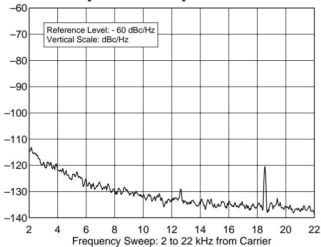
ICOM IC-706MkII G 01674 3.520 MHz, Phase Noise, 100 W F:\SHARED\PROD_REV\TESTS\IC706G\IC706P80.TXT
